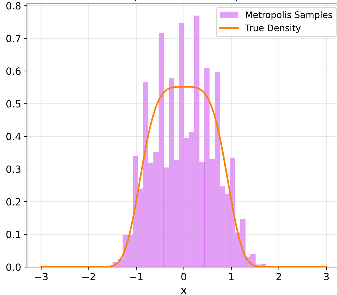
Random Walk (Step=0.075), Acceptance Rate=0.94
