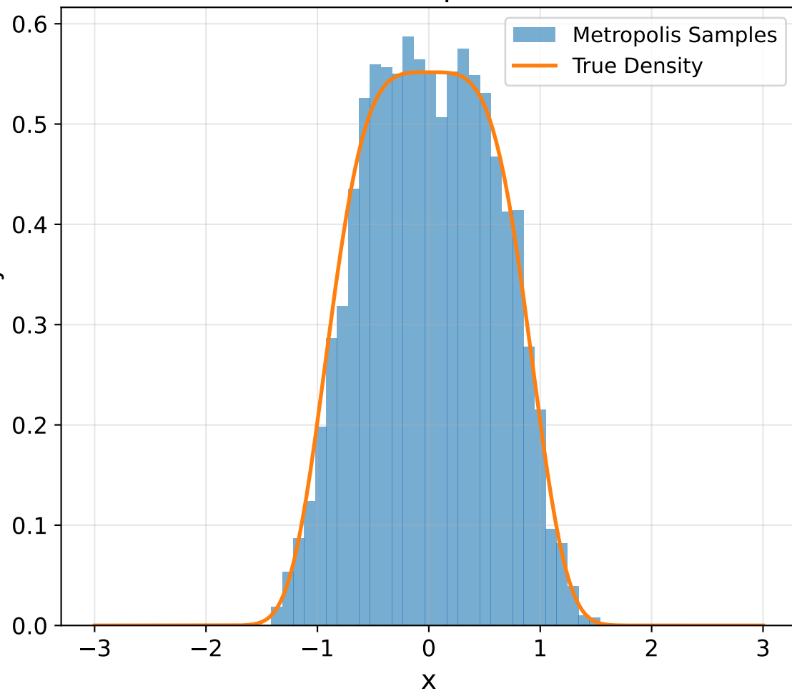
Uniform(-1, 1), Acceptance Rate=0.73
